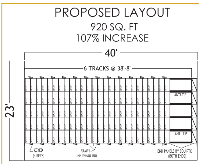
Pipp used existing shelving and converted it to Mobile Shelving which required 920 square feet. Pipp provided an additional 107% of storage capacity in the same amount of space!!
